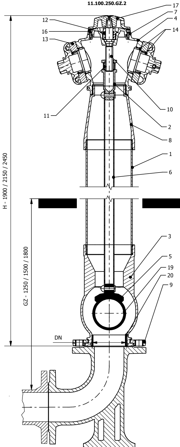
HN3 DN100 PN10/16 GJS 11.100.250.GZ.2
